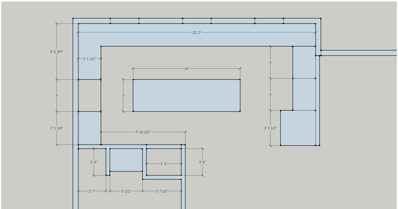
Kitchen Overview - Counter - Soapstone Total: 69.8 ft 2 ; weight 1,396 lbs. @ 20 lbs/ft 2 ; Island - Sapele Total: 30 ft 2 ; weight 158 lbs.
